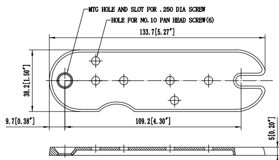
MOUNTING BRACKET (1) AND 10-32UNF X .250 REF PAN HEAD SCREW (2) FURNISHED UNASSEMBLED SCALE-HALF SIZE
