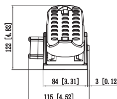
MTTNG CONNECTOR TE C-967616
